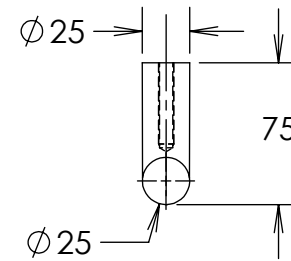
6200-25 SIDE VIEW
