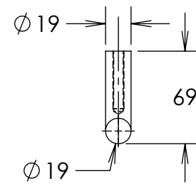
6200-19 SIDE VIEW
