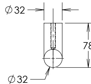
6200-32 SIDE VIEW
