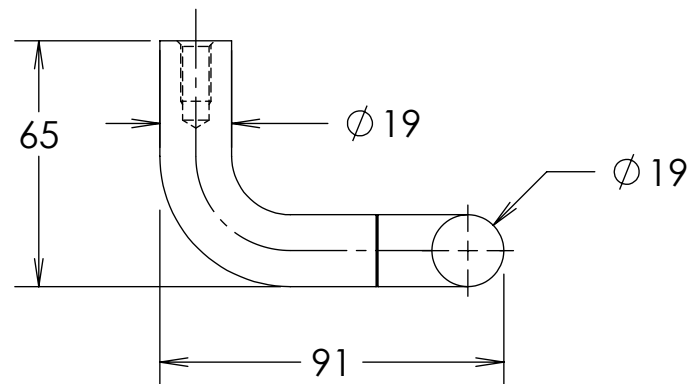
5250-19 SIDE VIEW
