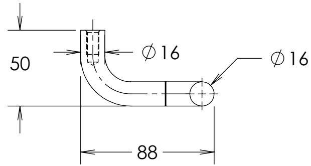
5250-16 SIDE VIEW
