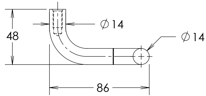
5250-14 SIDE VIEW
